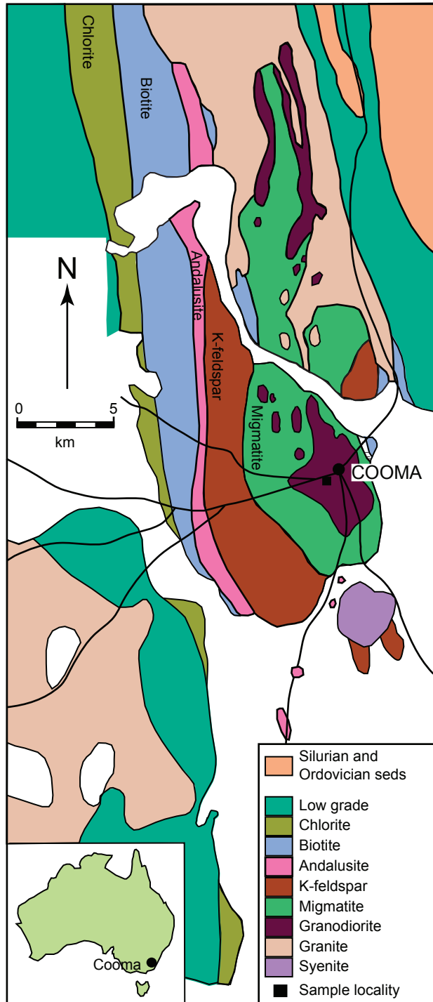
Fig. 3. Geologic and location maps for the Cooma granodiorite and the surrounding regional metamorphic zones in southeastern Australia. The location of the sample used in this study is also shown.
