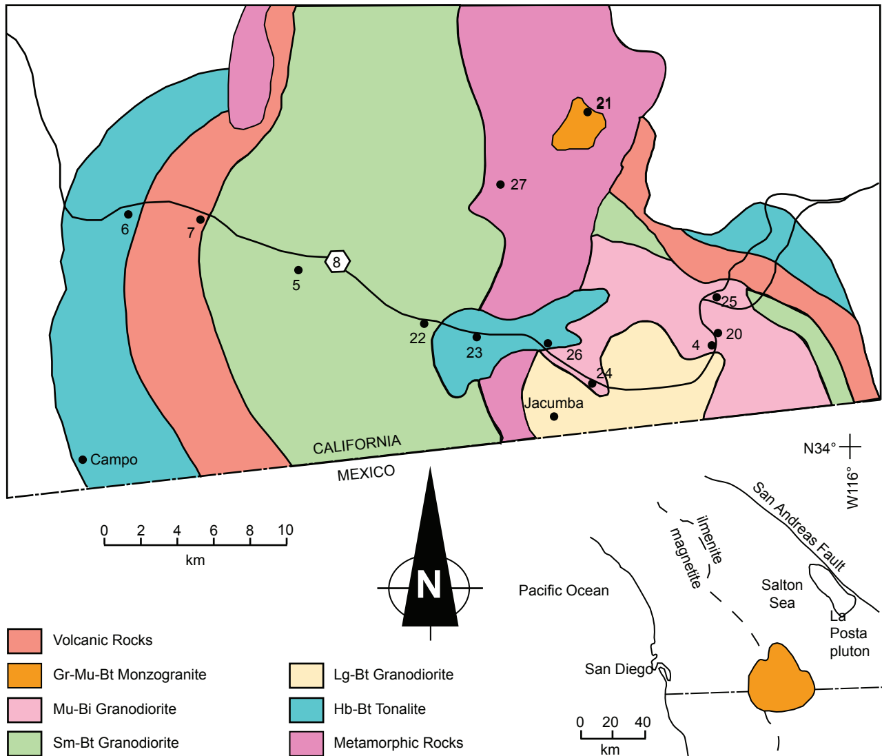
Fig. 2. Geologic and location maps for the La Posta pluton, Peninsular Ranges Batholith, southern California, showing the different facies of this zoned pluton and the sampling locations.
