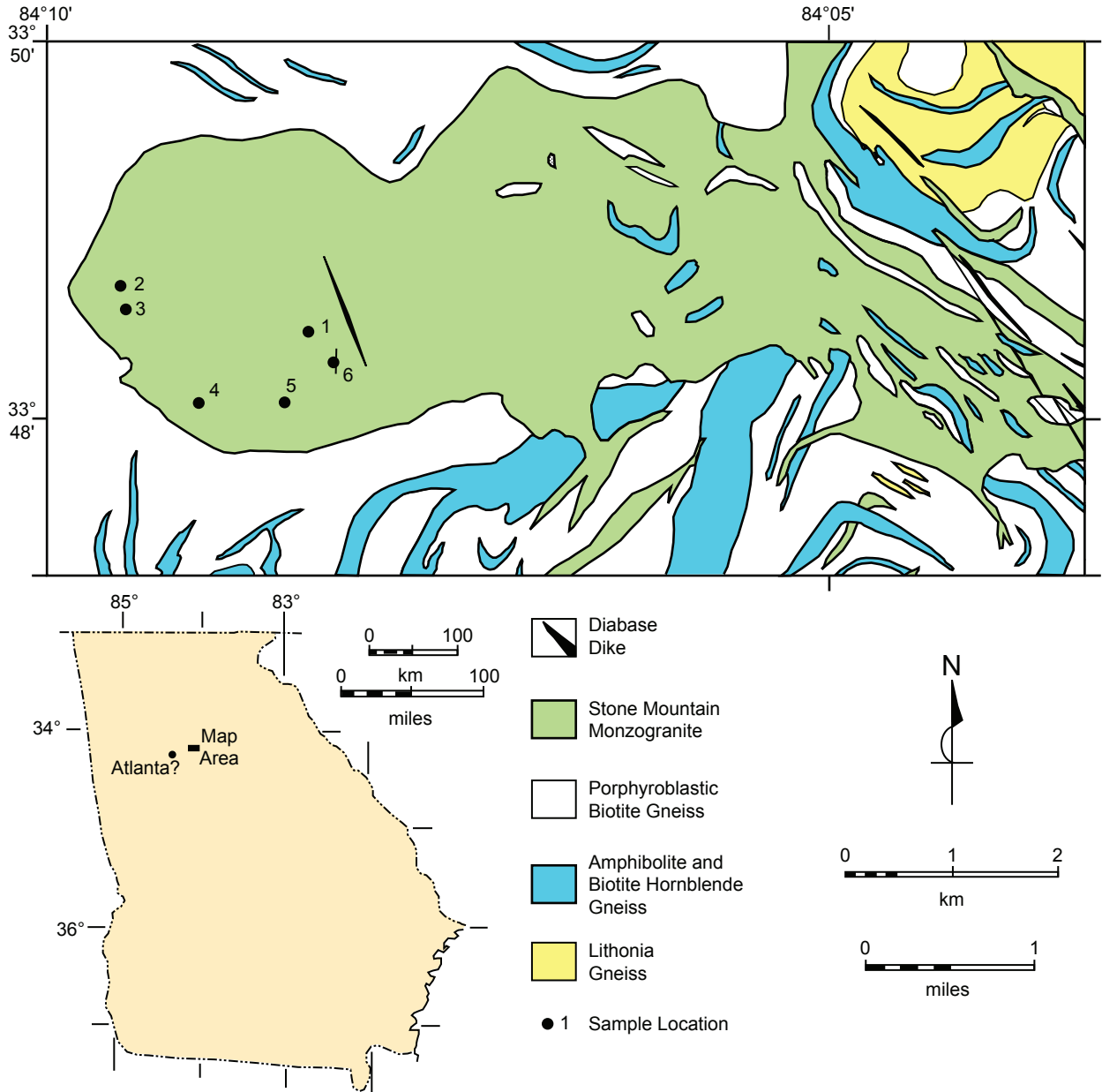
Fig. 1. Geologic map of the main area of the Stone Mountain pluton, showing its location near Atlanta, Georgia, and the locations of the samples examined for radiohalos.
