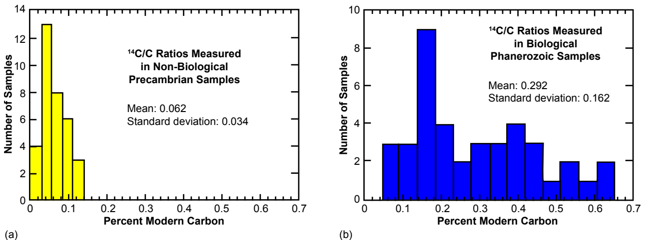
Fig. 2. Distribution of 14 C values for (a) non-biogenic samples and (b) biogenic samples from Table 1. Given their position in the geological record, all these samples should contain no detectable 14 C according to the standard geological time scale.
