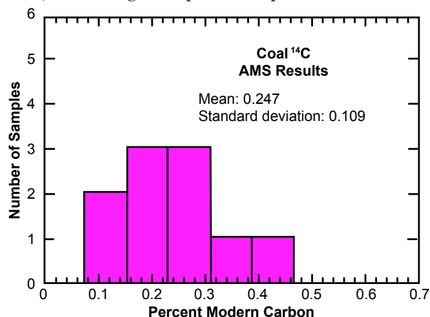
Fig. 3. Histogram representation of AMS ^{14}\text{C} analysis of ten coal samples undertaken by RATE ^{14}\text{C} research project.
