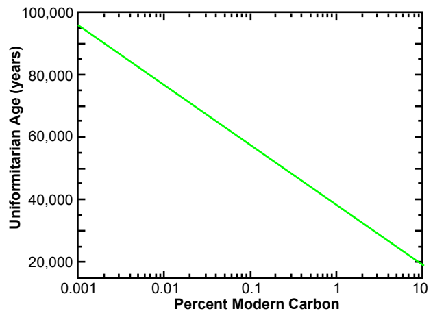
Fig. 1. Uniformitarian age as a function of ^{14}\text{C}/\text{C} ratio in percent modern carbon. The uniformitarian approach for interpreting the ^{14}\text{C} data assumes a constant ^{14}\text{C} production rate and a constant biospheric carbon inventory extrapolated into the indefinite past. It does not account for the possibility of a recent global catastrophe that removed a large quantity of carbon from the biospheric inventory.
