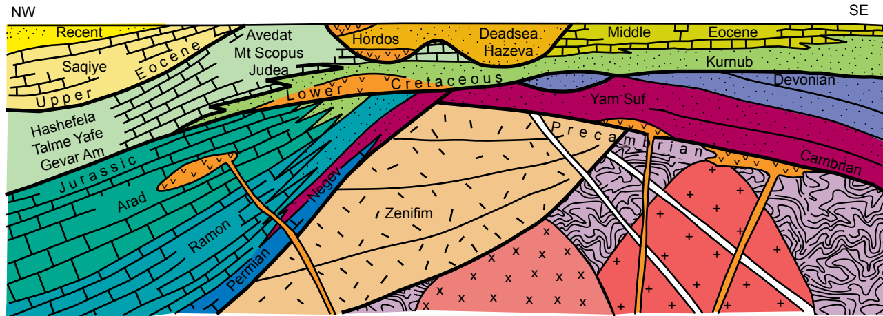
Fig. 11. The generalized stratigraphic sequence across Israel, extending from the Mediterranean coast in the northwest to Arabia in the southeast (after Freund 1977). The relationships between the major rock units of Israel's geology are depicted, with the heavy lines representing the regional unconformities separating six major stratigraphic "packages" of strata. The conventional ages of the tops and bottoms of these strata "packages" are designated. Dotted areas indicate clastic rocks; bricks indicate shales and non-clastic (mainly calcareous) rocks; vs indicate volcanics.
