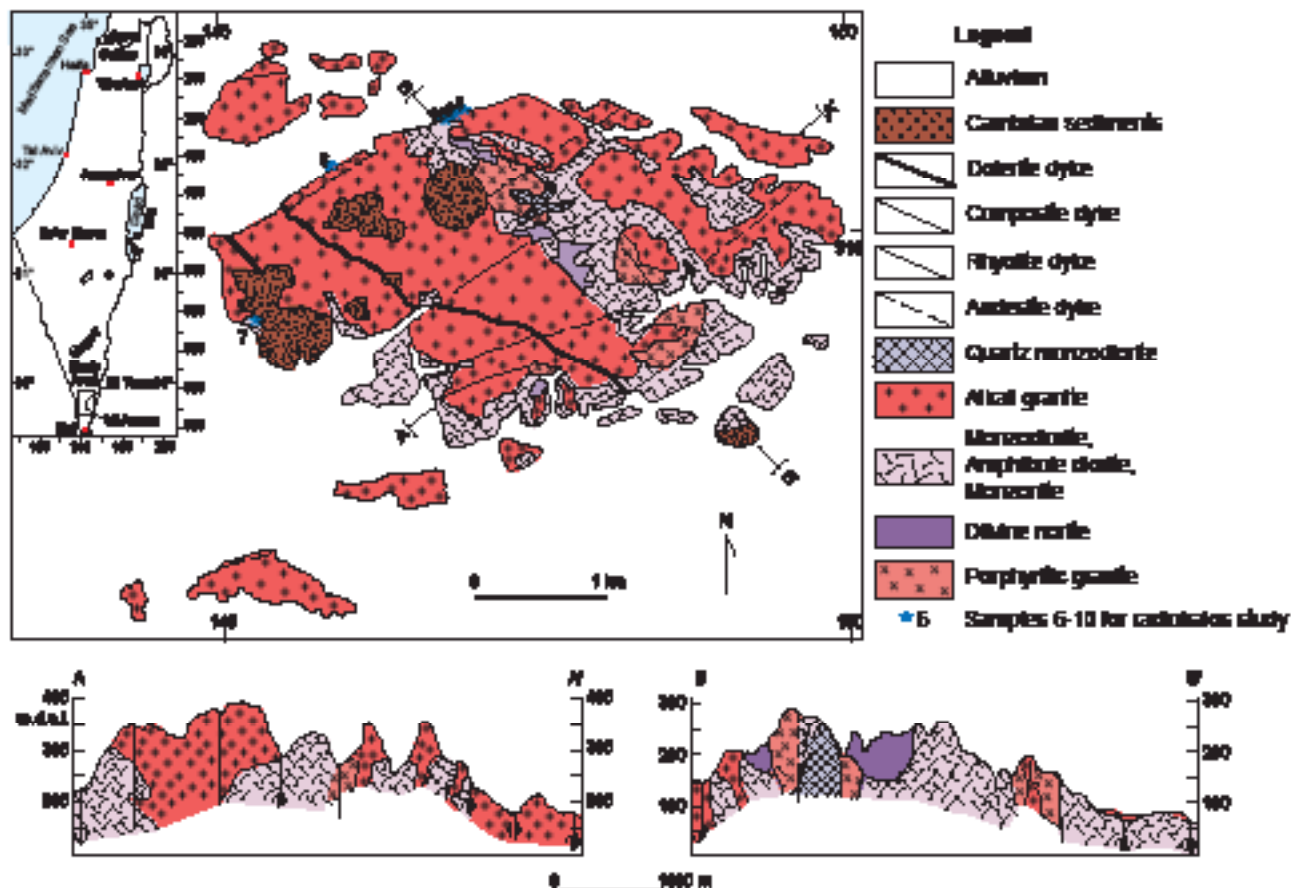
Fig. 6. Location and general geologic maps of, with two geologic cross-sections through, the Timna Igneous Complex in the Mt. Timna area of southernmost Israel (after Beyth et al. 1994a). The locations of the samples collected for the radiohalos study are shown.
